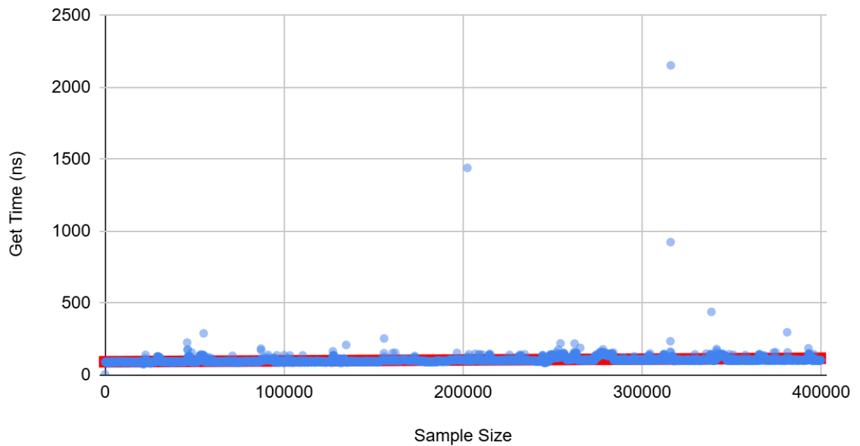
Get Time (nanoseconds) vs. Sample Size
