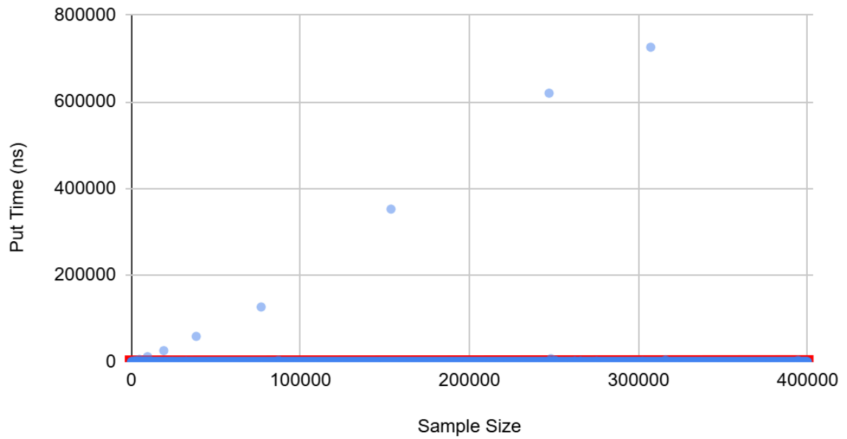
Put Time (nanoseconds) vs. Sample Size
